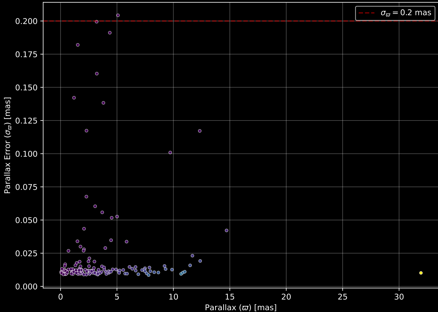
APOGEE DR17 Field: [055+36_MGA] Parallax Quality (n= 169)
