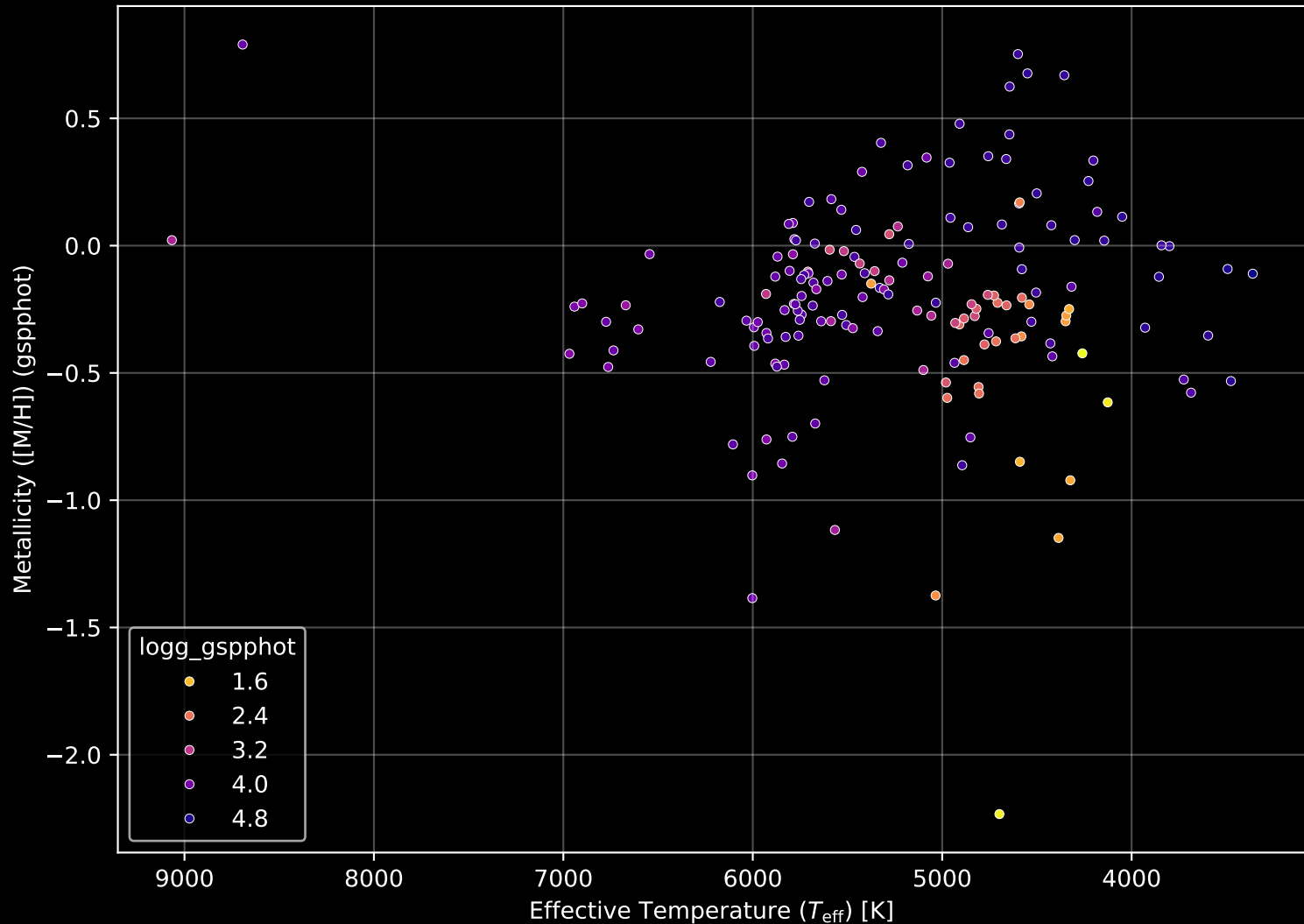
APOGEE DR17 Field: [055+36_MGA] Stellar Population Parameters (n= 169)
