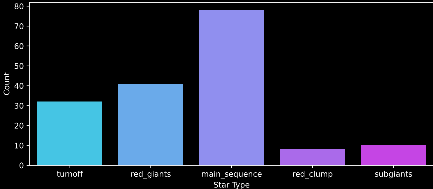
APOGEE DR17 Field: [055+36_MGA] Count plot of Star Type
