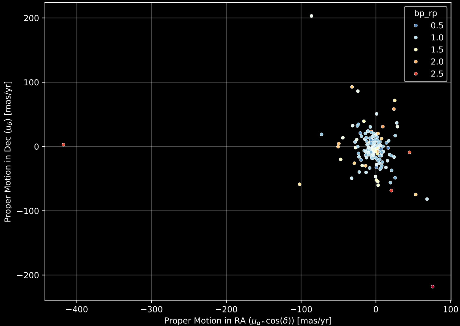
APOGEE DR17 Field: [055+36_MGA] Proper Motion Diagram (n= 169)
