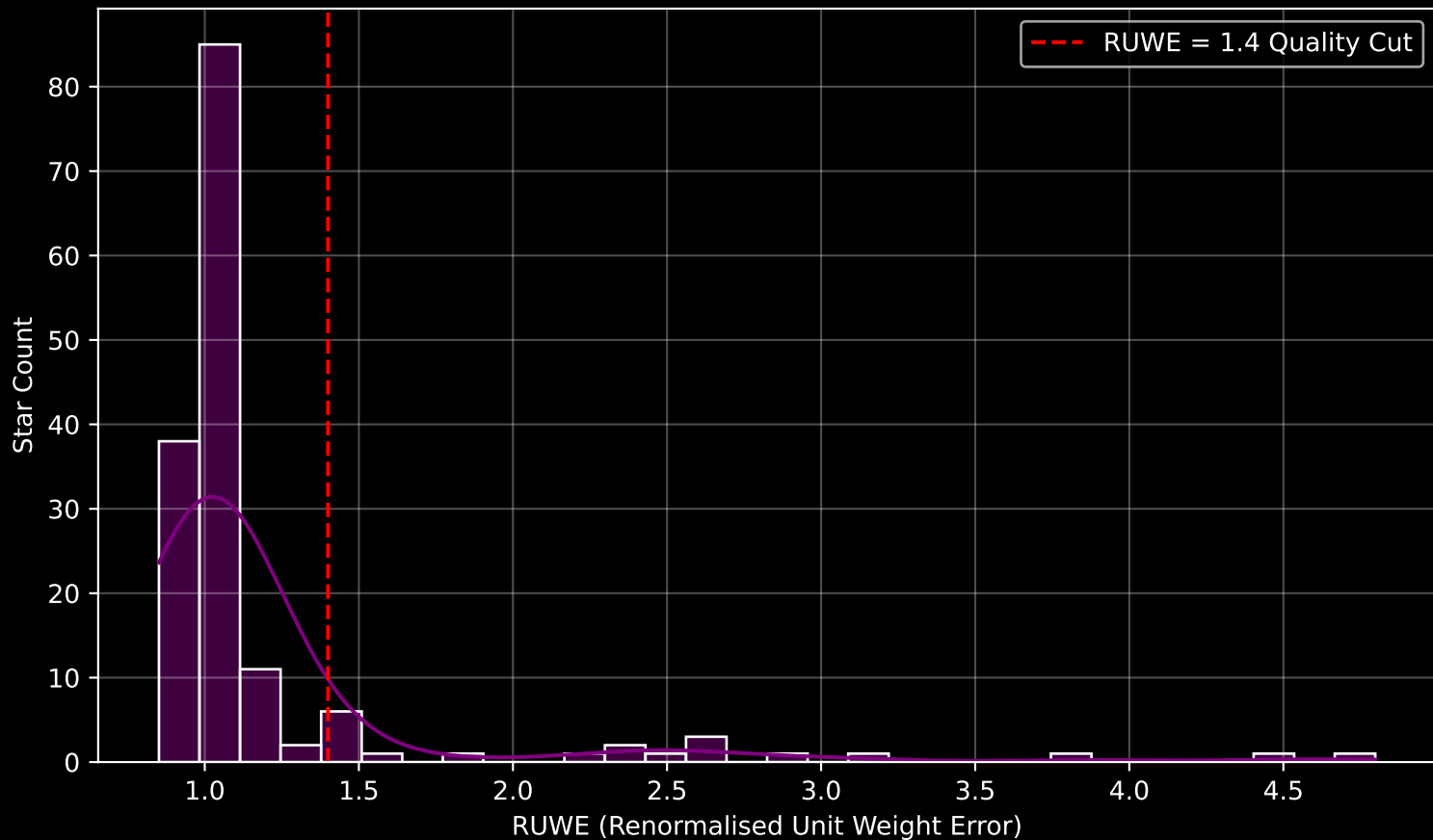
GAPOGEE DR17 Field [055+36_MGA] RUWE Distribution (n= 156)
