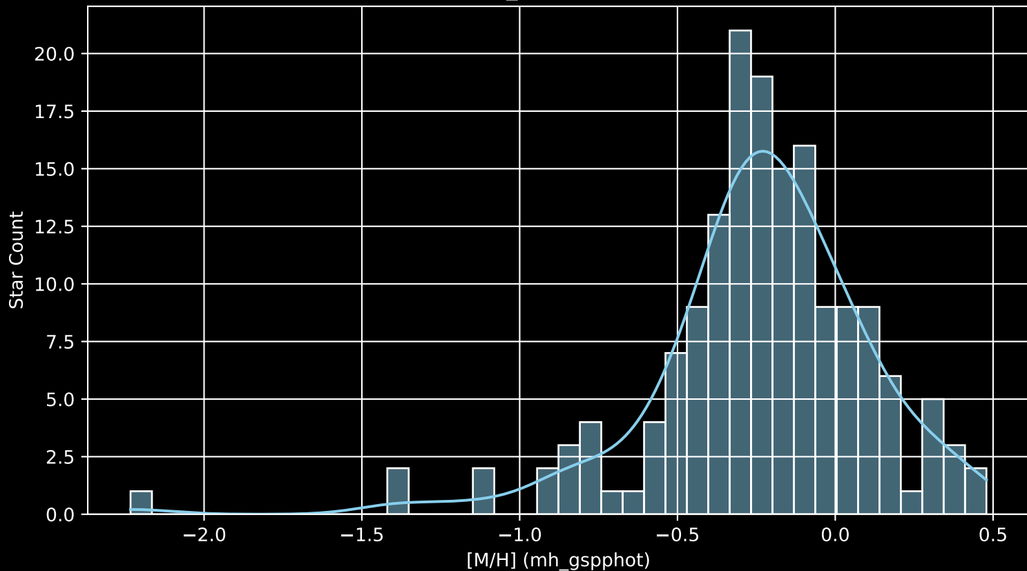
APOGEE DR17 Field: [055+36_MGA [M/H] (mh_gspphot) (n= 164)
